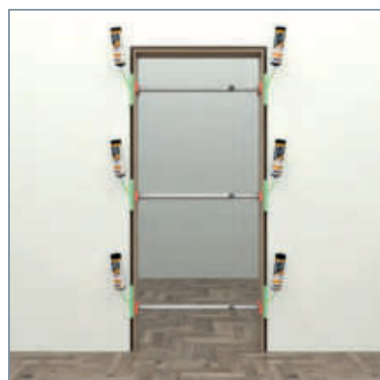
2. Foam with 2-component PU foam.
